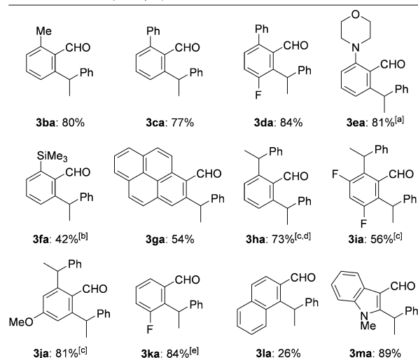
Scheme 2. Addition of various aromatic aldimines to styrene (0.3 mmol scale). The branched/linear ratio was greater than 50:1. Unless otherwise stated the yields are those of the isolated products. [a] A 0.9 mmol scale. [b] The yield was determined by 1 H NMR spectroscopy using 1,1,2,2-tetrachloroethane as an internal standard. [c] The reaction was performed using 2.4 equiv of styrene. The product was obtained as an approximately 1:1 mixture of diastereomers. [d] The product obtained as a mixture with the monoadduct (7%). [e] The reaction was performed using 0.3 mmol of aldimine and 0.12 mmol of styrene. The yield was based on styrene.
