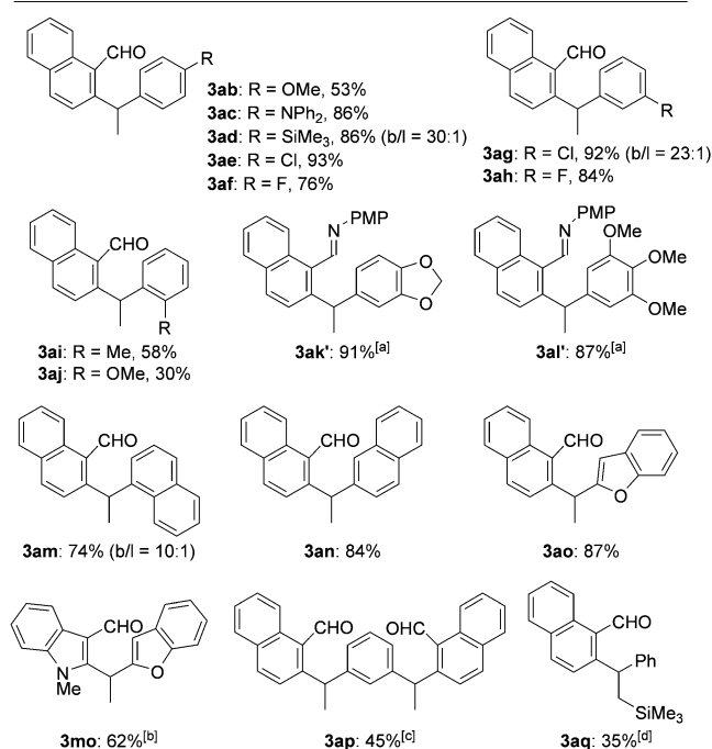
Scheme 3. Addition of 1a to various styrene derivatives (0.3 mmol scale). The branched/linear ratio was greater than 50:1 unless otherwise noted. The yields are those of the isolated products. [a] The product was obtained without acidic hydrolysis. [b] The aldimine derived from indole-3-carboxaldehyde ( 1l ) was used instead of 1a . [c] The reaction was performed using 3 mmol of 1a , 1.2 mmol of 1,3-divinylbenzene, 20 mol % of CoBr 2 , 40 mol % of P( p -Tol) 3 , and 100 mol % of Me 3 SiCH 2 MgCl. The product was obtained as an approximately 1:1 mixture of diastereomers. [d] The reaction was performed using (Z)-trimethyl(styryl)silane.
